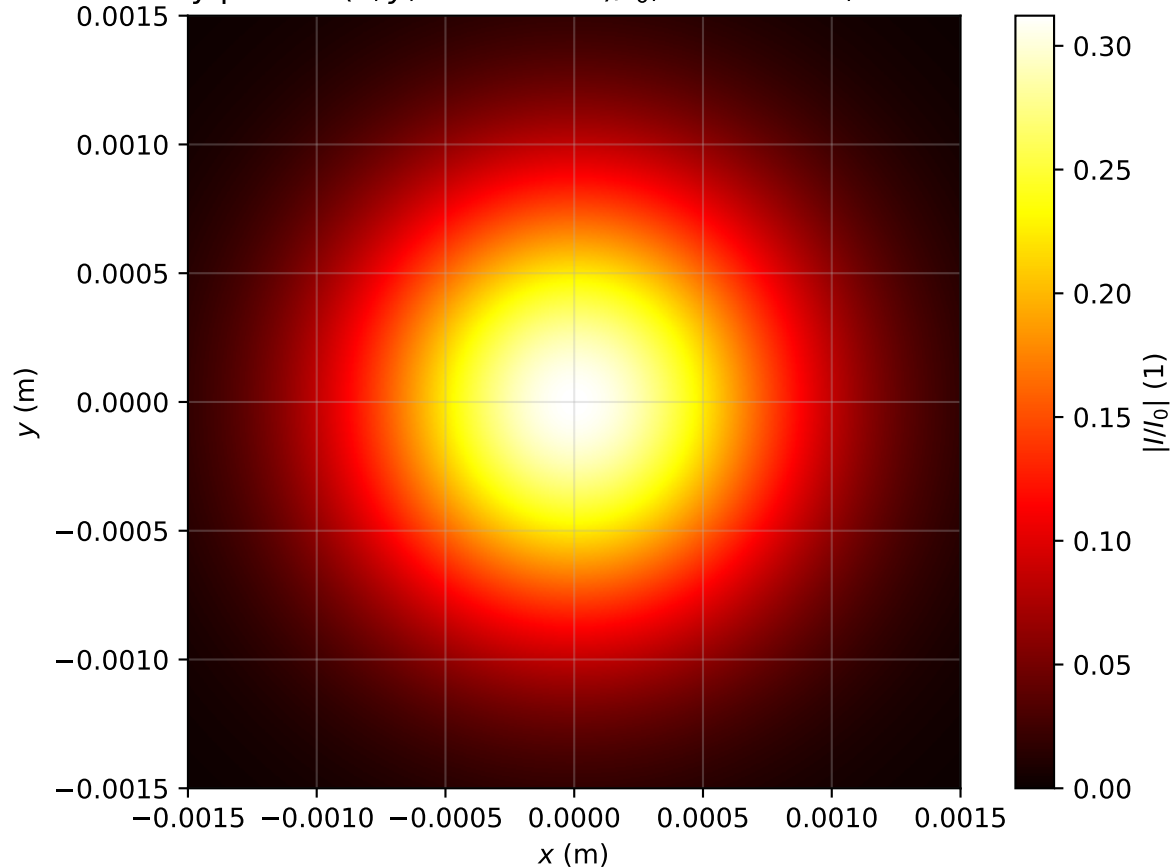
Intensity profile I(x, y, z = 3.423m)/I_0 , P_{in}=0.2P_{cr} , artificial time
